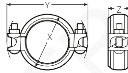
Joint Assembled
